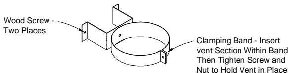
FIG. 7 WALL BRACKET/SUPPORT
