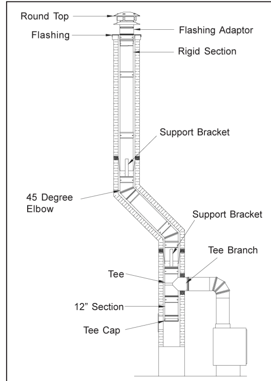
Standard installation of the Rigid Stainless Steel Liner with offset
