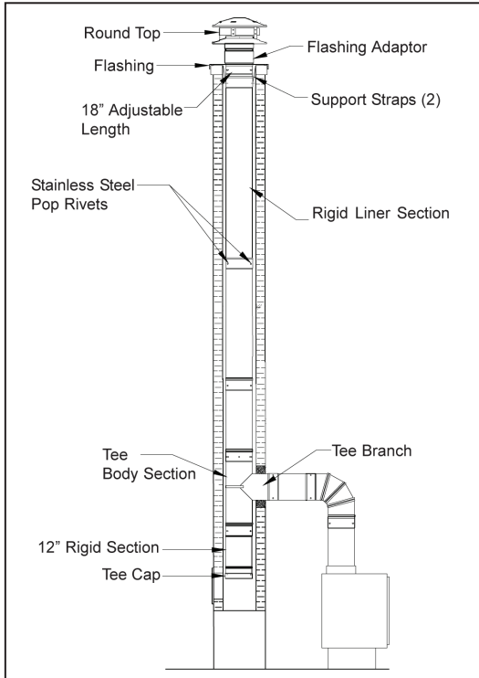
Standard installation of the Rigid Stainless Steel Liner
