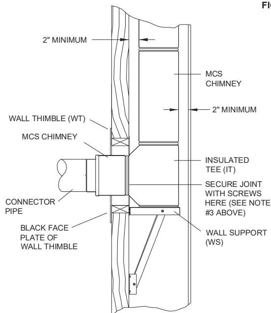
WALL THIMBLE/ CHIMNEY COMPLETED ASSEMBLY
