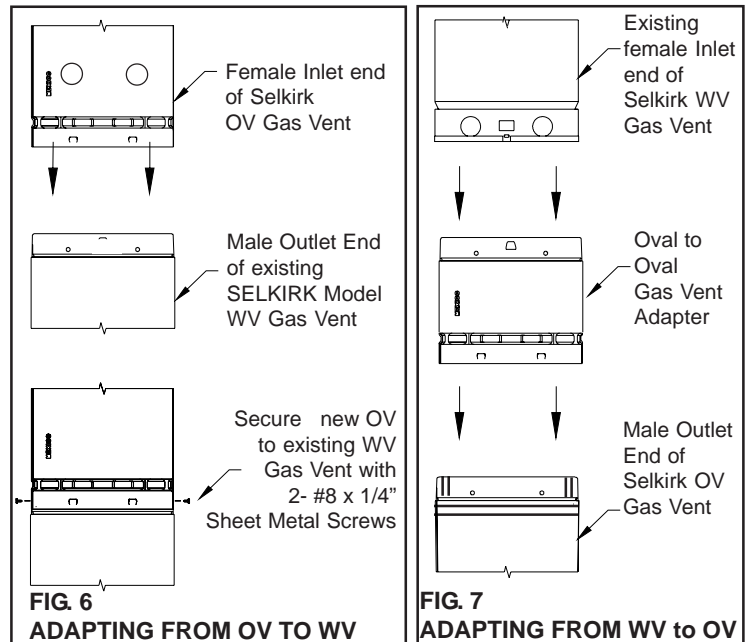
Illustration 5 - Adding Selkirk Oval Gas Vent
