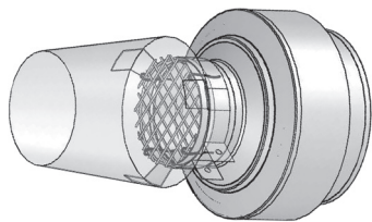
4DT-VP0S Outlet Screen installed
