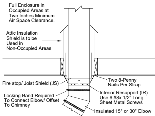
FIG 8 - INTERIOR RESUPPORT (IR) USE WHEN THE INSTALLATION OF AN INTERIOR RESUPPORT BELOW A LOCKING BAND IS NOT POSSIBLE
