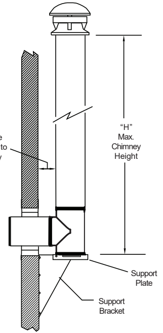
FIG. 3 - See Table 2 for Maximum Chimney Heights based upon Chimney Diameter and Distance from Wall
