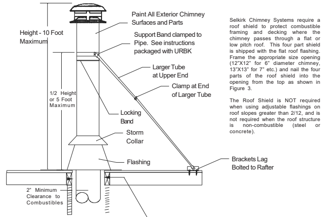
FIG. 3 ROUND CHIMNEY BRACING REQUIREMENTS USING 6", 7", OR 8" ROOF BRACE KIT OR EQUIVALENT METHOD
